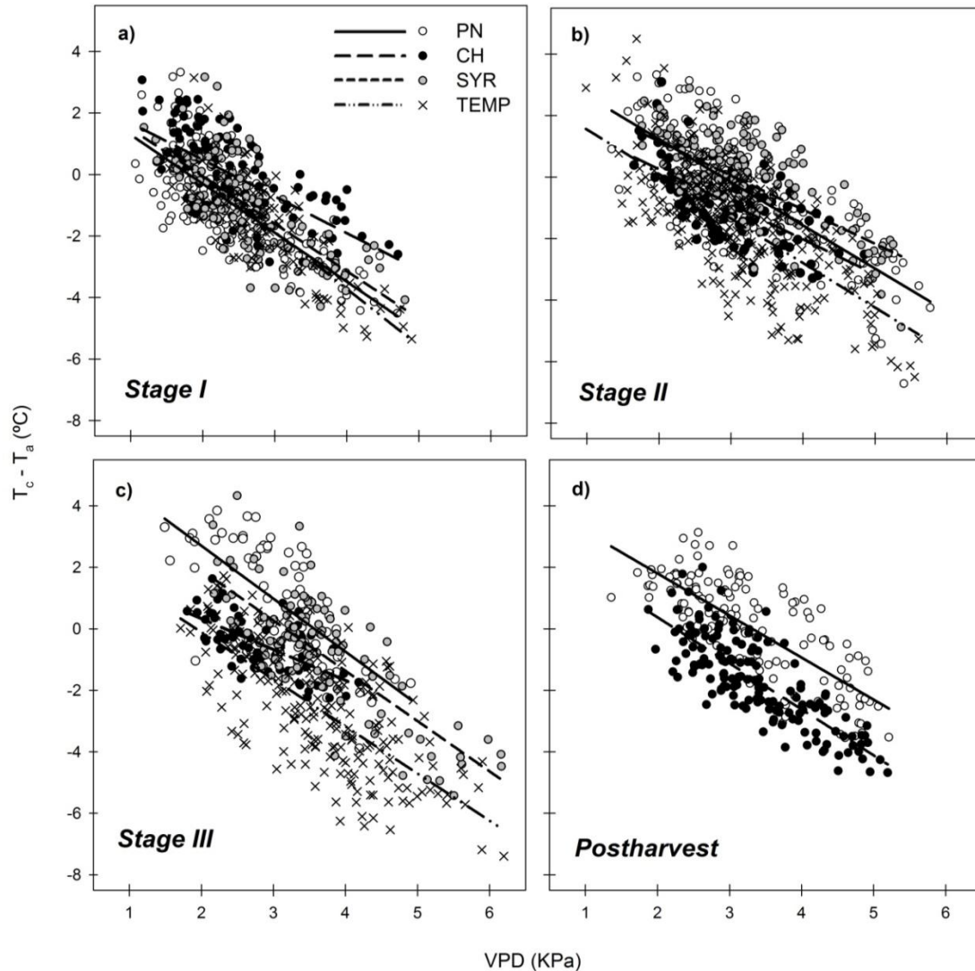
Figure 3.3. Differences between varieties Pinot-noir (PN), Chardonnay (CH), Syrah (SYR) and Tempranillo (TMP) in the relationship between difference of canopy and air temperature ( T_c - T_a ) and vapour pressure deficit (VPD) at different phenological stages (Stage I, II, III and post-harvest). Equations and coefficients of determination ( r^2 ) are: Stage I; PN: y = -1.592x + 2.885 , r^2 = 0.553 ; CH: y = -1.194x + 2.869 , r^2 = 0.437 ; SYR: y = -1.542x + 3.027 , r^2 = 0.521 ; TMP: y = -1.848x + 3.675 , r^2 = 0.649 . Stage II; PN: y = -1.403x + 4.043 , r^2 = 0.524 ; CH: y = -1.138x + 2.529 , r^2 = 0.401 ; SYR: y = -1.026x + 3.066 , r^2 = 0.457 ; TMP: y = -1.479x + 3.107 , r^2 = 0.489 . Stage III; PN: y = -1.722x + 6.146 , r^2 = 0.469 ; CH: y = -1.004x + 2.335 , r^2 = 0.426 ; SYR: y = -1.576x + 4.929 , r^2 = 0.565 ; TMP: y = -1.449x + 2.685 , r^2 = 0.515 . Post-harvest; PN: y = -1.367x + 4.536 , r^2 = 0.575 ; CH: y = -1.540x + 3.535 , r^2 = 0.667 . All relationships were significant ( p < 0.0001 ).
