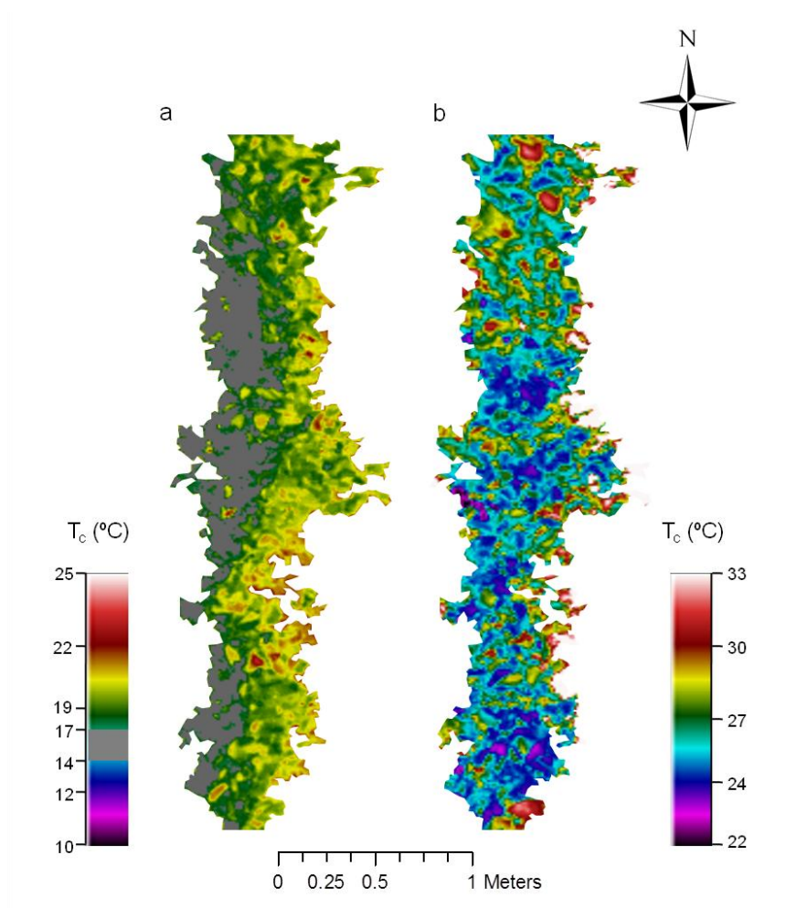
Figure 2.8. Example of the shading effect on the canopy temperature ( T_c ) at two different times of the day: a) 08:00 h and b) 12:00 h. Air temperatures ( T_a ) at 08:00 and 12:00 hours were 18.5 and 25 °C, respectively. Rows are orientated north-south.
