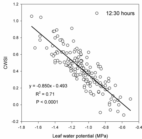
Figure 2.6. Relationship between CWSI and midday leaf water potential ( \Psi_L ) measured in 184 vines of 'Pinot-noir' vineyard at 12:30 h. CWSI was obtained from thermal camera imagery from an unmanned aerial vehicle (UAV).
