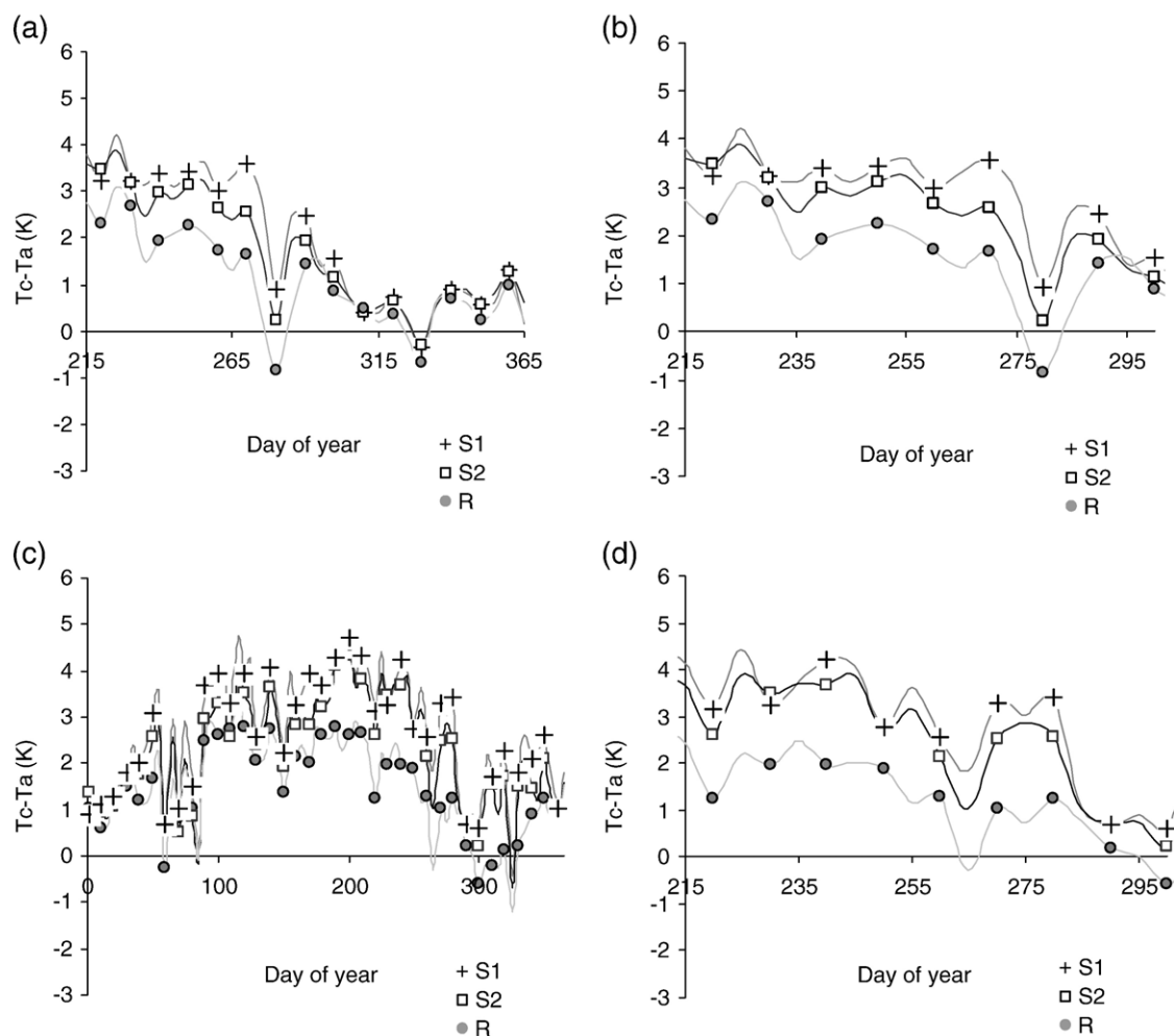
Fig. 4. Yearly T_c - T_a (K) differences at 14:00 GMT for the different olive irrigation treatments. T_c and T_a were measured with the infrared thermal sensors placed on top of the olive trees. a) From July to December 2004, b) data for the summer 2004, c) from January to December 2005, and d) data for summer 2005.
