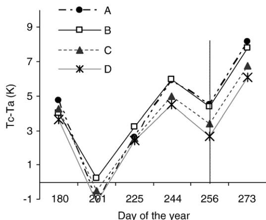
Fig. 3. Differences between canopy ( T_c ) and air ( T_a ) temperature (K) for the different irrigation treatments obtained with a hand-held infrared thermometer at 12:00 GMT from peach trees in the 2005 summer campaign. Irrigation period ended on 13 September (day 256, dashed line).
