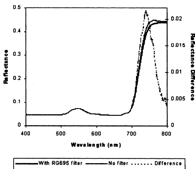
FIGURE 1. Single leaf reflectance measurements obtained with the Li-Cor 1800 apparatus and fibre spectrometer using the measurement protocol with the RG695 filter (thick line) and with no filter (thin line) from a dark-adapted Acer saccharum M. leaf sample [adapted from Zarco-Tejada et al 2000a].
