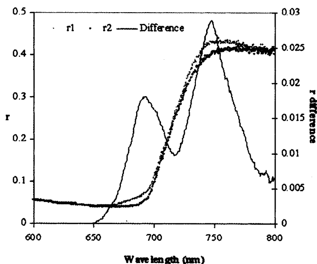
FIGURE 2. Reflectance measurements taken at t_0 ( r_1 ) and t_1 (5 min) ( r_2 ) in a time-decay experiment which demonstrates the effect of fluorescence emission bands on the reflectance spectra in the 600-800 nm spectral region due to PSII and PSI photosystems
