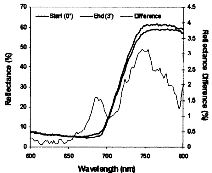
FIGURE 4. Effect of the CF variation in a time-decay experiment in the 600-800 nm canopy reflectance. CASI canopy reflectance measurements were made from Acer saccharum M. seedlings in the laboratory taken after dark adaptation and after 3 minutes of illumination. Differences in reflectances at 680-690 nm and 730-750 nm are observed due to changes in chlorophyll fluorescence.
